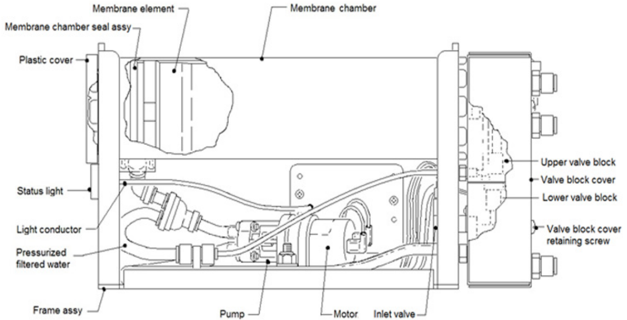
Fig. 9a: Right hand side view of unit with the outer cover removed
