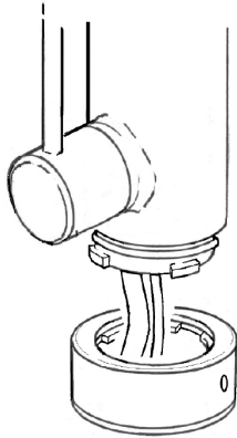
Fig.14a: Placing faucet on mounting socket
