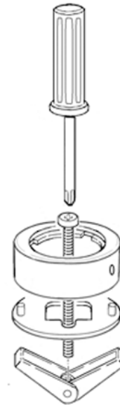
Fig. 13b: Pre assembly of mounting socket
